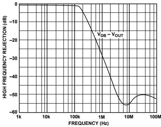
Figure 44. Frequency Response of Filter
