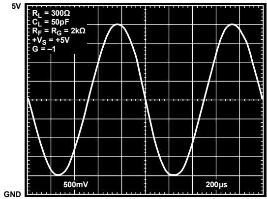
Figure 29. Output Swing, +V_S = +5\text{V} , G = -1
