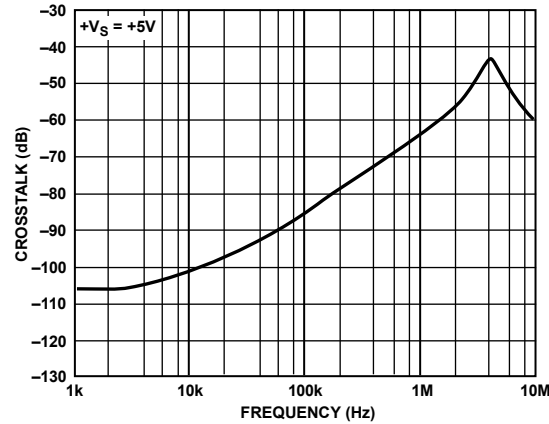
Figure 27. Crosstalk vs. Frequency
