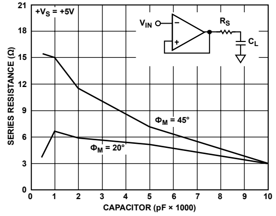
Figure 26. Series Resistance vs. Capacitive Load
