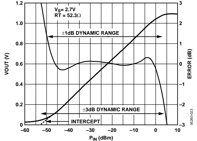
Figure 23. VOUT and Log Conformance Error vs. Input Level vs. Input Level at 900 MHz
