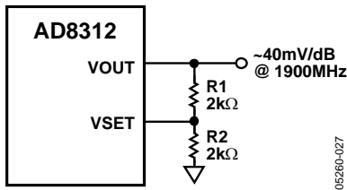
Figure 27. Increasing the Output Slope
