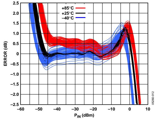
Figure 12. Distribution of Error at -40^{\circ}\text{C} , +25^{\circ}\text{C} , and +85^{\circ}\text{C} After Ambient Normalization vs. Input Amplitude at 1.9 GHz for 80 Devices
