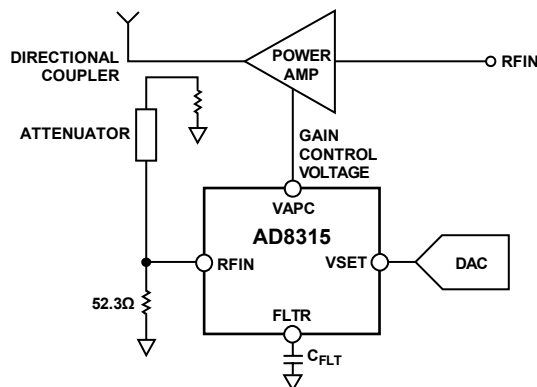
Figure 37. Typical Application
