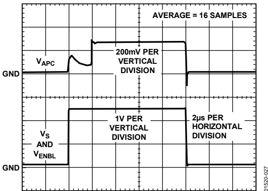
Figure 27. Power-On and Power-Off Response with VSET Grounded
