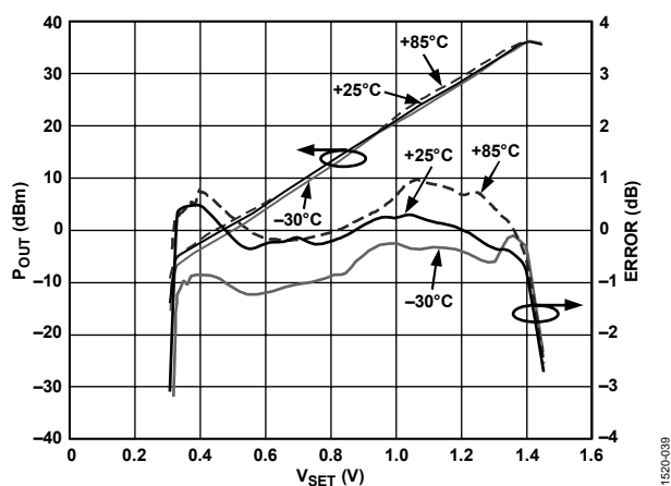
Figure 39. P_{OUT} vs. V_{SET} at 0.9 GHz for Dual-Mode Handset Power Amplifier Application, -30^{\circ}\text{C} , +25^{\circ}\text{C} , and +85^{\circ}\text{C}
