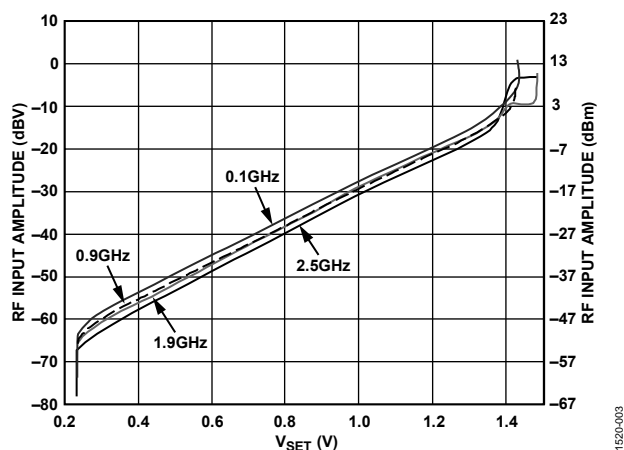
Figure 3. Input Amplitude vs. V_{SET}
