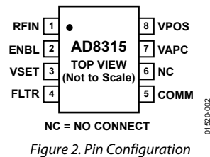
Figure 2. Pin Configuration
