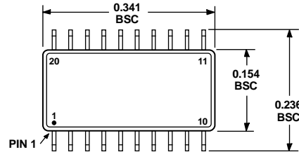
Figure 30. 20-Lead Lead Frame Chip Scale Package [LFCSQ_VQ]
