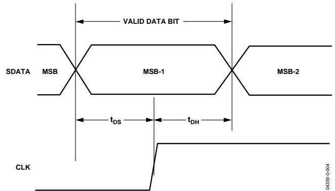
Figure 4. SDATA Timing
