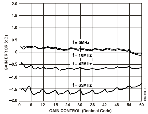
Figure 18. Gain Error vs. Gain Control
