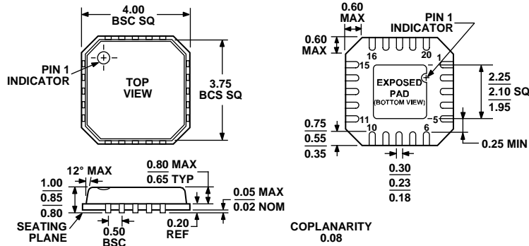
Figure 30. 20-Lead Lead Frame Chip Scale Package [LFCSQ_VQ]
