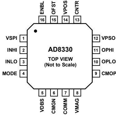
Figure 2. 16-Lead LFCSP Pin Configuration
