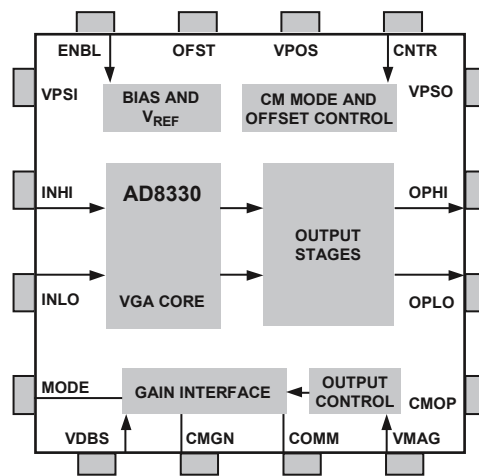
Figure 46. Block Schematic
