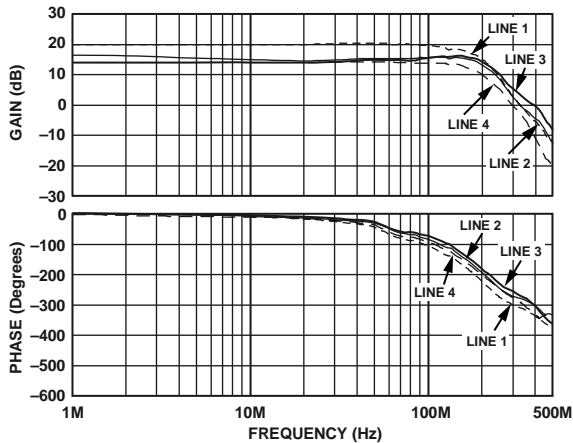
Figure 60. AC Gain and Phase for Various Loading Conditions
