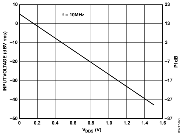
Figure 28. Input Voltage 1 dB vs. V_{DBS}
