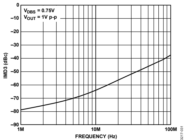
Figure 30. IM3 Distortion vs. Frequency
