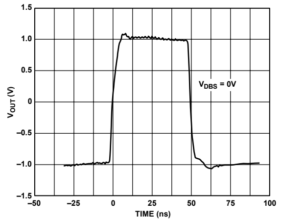
Figure 33. Full-Scale Transient Response, V_{DBS} = 0V
