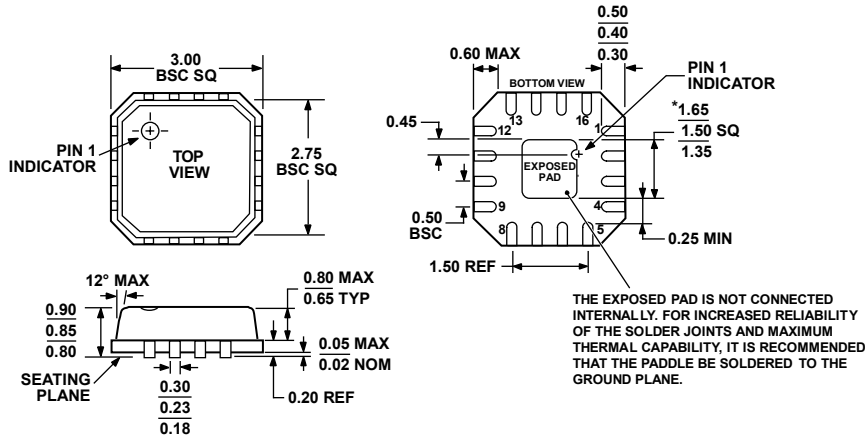
Figure 69. 16-Lead Lead Frame Chip Scale Package [LFCSP_VQ] 3 mm x 3 mm Body, Very Thin Quad (CP-16-3) Dimensions shown in millimeters
