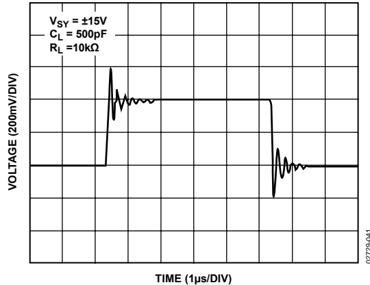
Figure 46. Capacitive Load Drive Without Snubber
