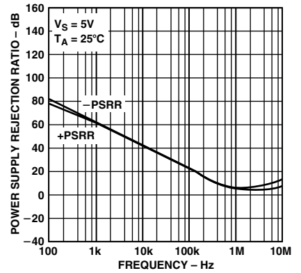
TPC 15. Power Supply Rejection Ratio vs. Frequency
