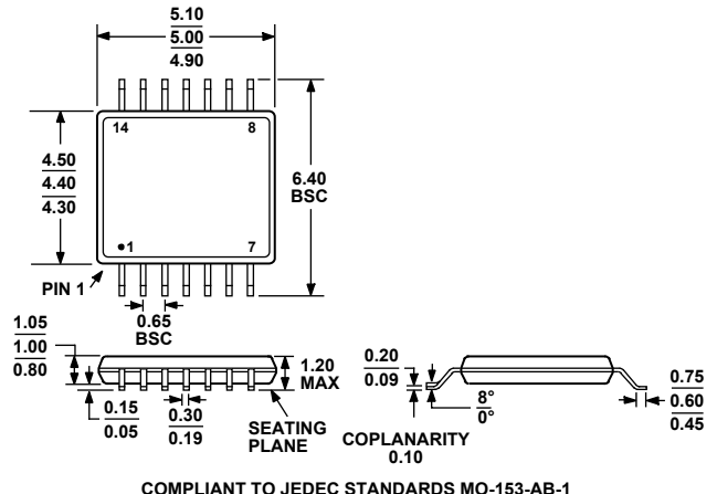
Figure 41. 14-Lead Thin Shrink Small Outline Package [TSSOP] (RU-14)
