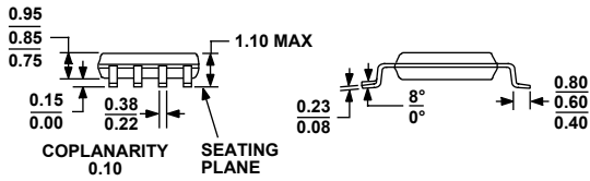
Figure 44. 8-Lead Mini Small Outline Package [MSOP] (RM-8)
