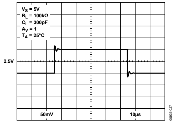
Figure 27. Small Signal Transient Response
