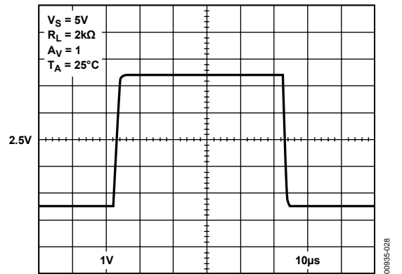
Figure 28. Large Signal Transient Response
