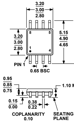
Figure 45. 8-Lead Mini Small Outline Package [MSOP] (RM-8)
