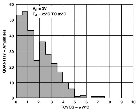
TPC 3. Input Offset Voltage Drift Distribution
