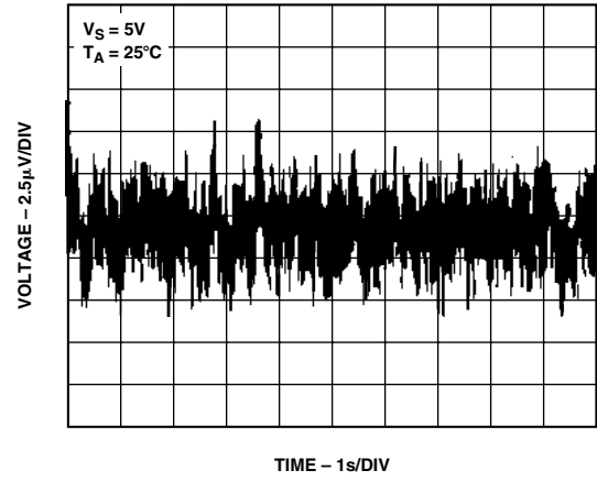
TPC 40. 0.1 Hz to 10 Hz Input Voltage Noise
