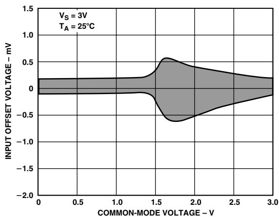
TPC 5. Input Offset Voltage vs. Common-Mode Voltage
