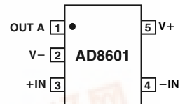
5-Lead SOT-23 (RT Suffix)
