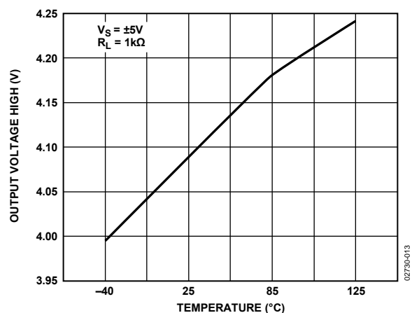
Figure 13. Output Voltage High vs. Temperature at \pm 5V
