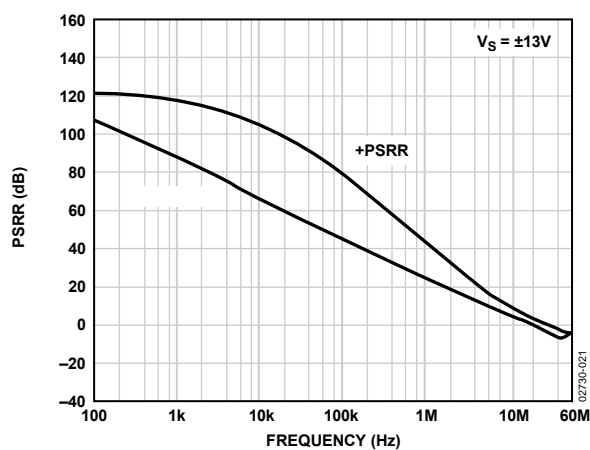
Figure 21. PSRR vs. Frequency at \pm 13\text{ V}
