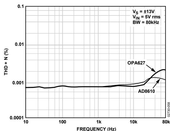
Figure 58. AD8610 vs. OPA627 THD + Noise @ V_{CM} = 0 V
