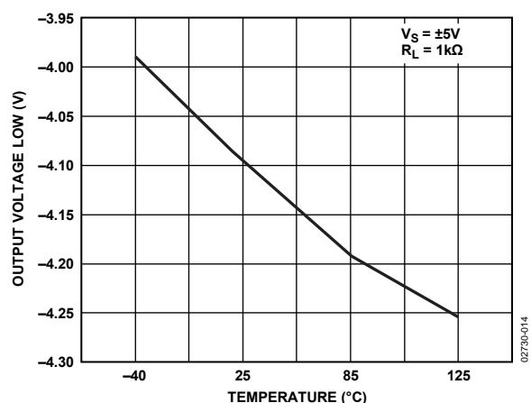
Figure 14. Output Voltage Low vs. Temperature at \pm 5V
