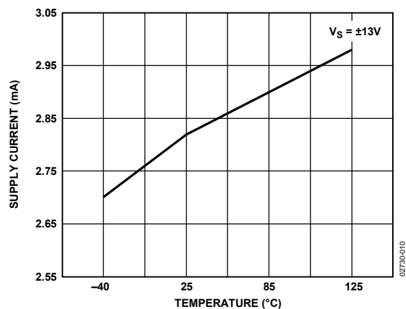
Figure 10. Supply Current vs. Temperature at \pm 13V
