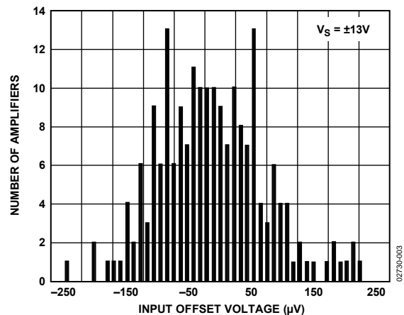
Figure 3. Input Offset Voltage at \pm 13 V
