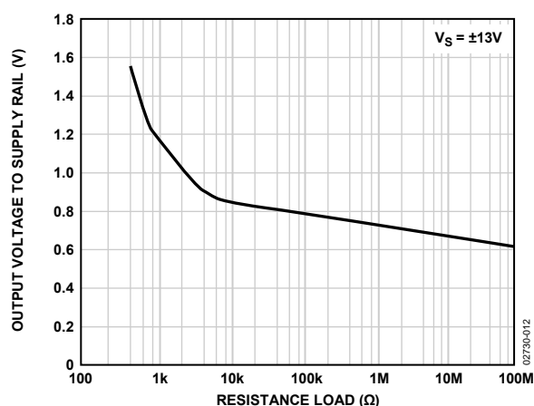
Figure 12. Output Voltage to Supply Rail vs. Load
