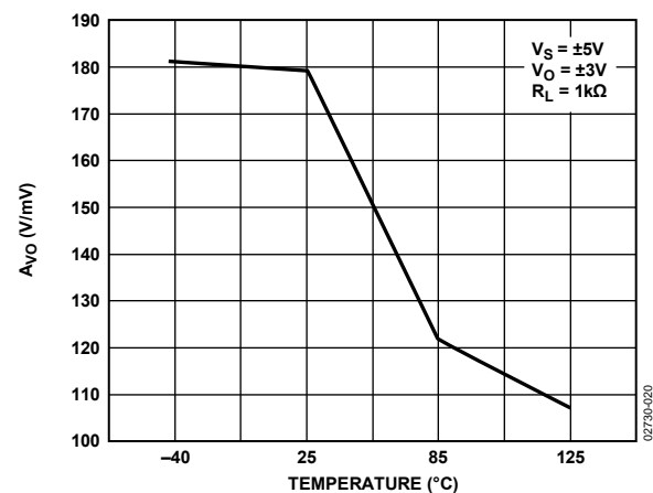
Figure 20. A_{VO} vs. Temperature at \pm 5 V
