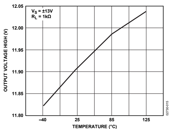
Figure 15. Output Voltage High vs. Temperature at \pm 13 V
