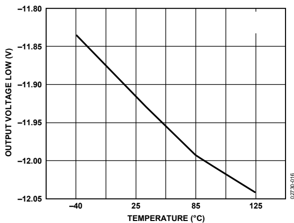
Figure 16. Output Voltage Low vs. Temperature at \pm 13 V
