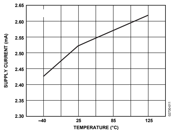
Figure 11. Supply Current vs. Temperature at \pm 5V
