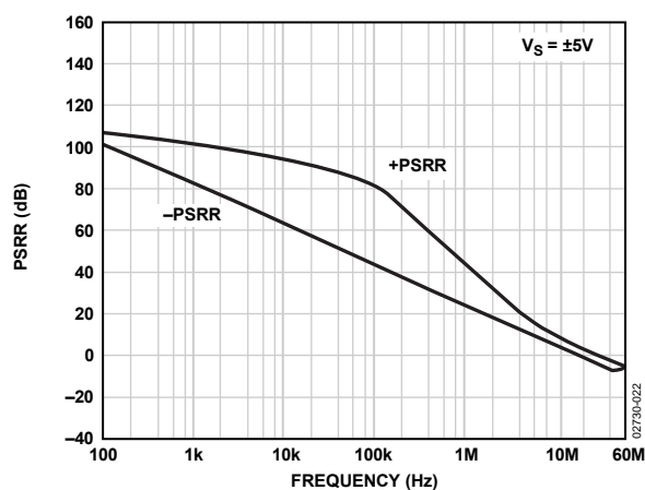
Figure 22. PSRR vs. Frequency at \pm 5\text{ V}
