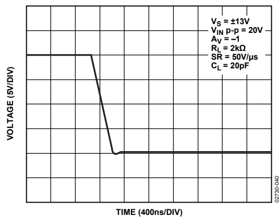
Figure 40. -SR at G = -1
