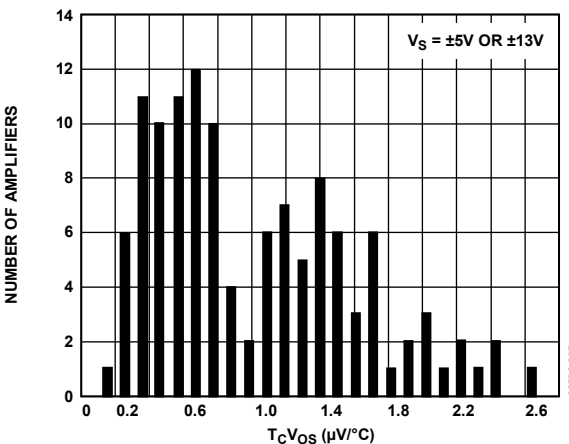
Figure 7. Input Offset Voltage Drift
