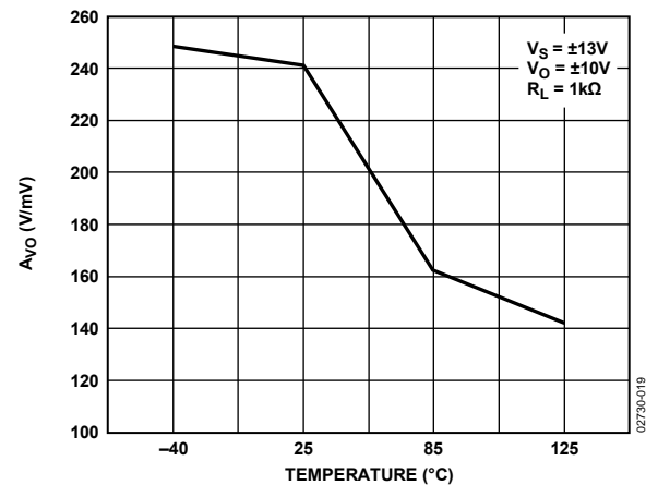
Figure 19. A_{VO} vs. Temperature at \pm 13 V
