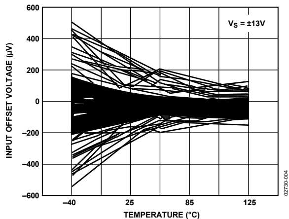
Figure 4. Input Offset Voltage vs. Temperature at \pm 13 V (300 Amplifiers)
