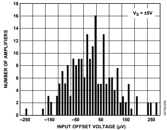
Figure 5. Input Offset Voltage at \pm 5 V
