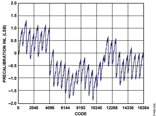
Figure 6. AD9117 Precalibration INL at 1.8 V, 8 mA
