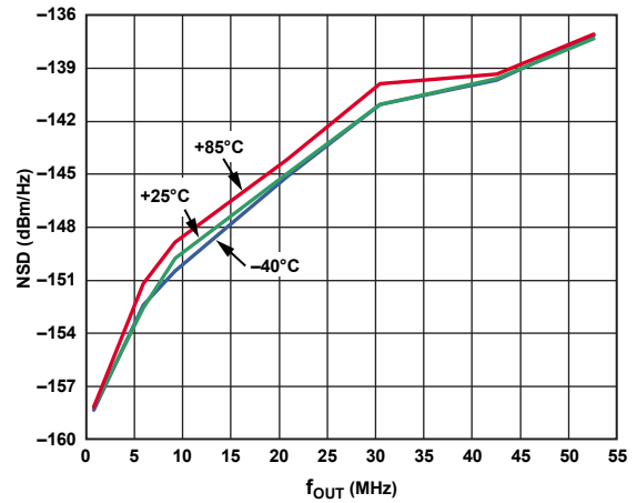
Figure 64. NSD at 8 mA, 1.8 V
