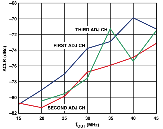
Figure 38. AD9117 Close In ACLR at 3.3 V, 20 mA
