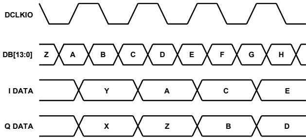
Figure 77. Timing Diagram with IFIRST = 0, IRISING = 1
