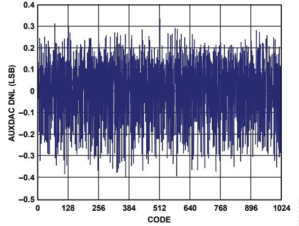
Figure 40. AUXDAC DNL
