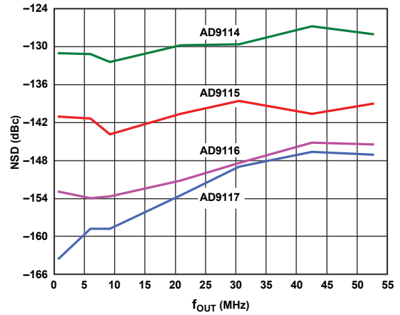
Figure 63. NSD at 20 mA, 3.3 V
