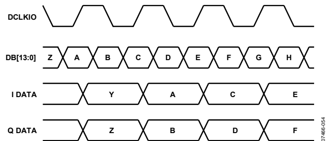
Figure 79. Timing Diagram with IFIRST = 1, IRISING = 1
