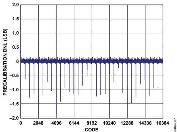
Figure 7. AD9117 Precalibration DNL at 1.8 V, 8 mA
