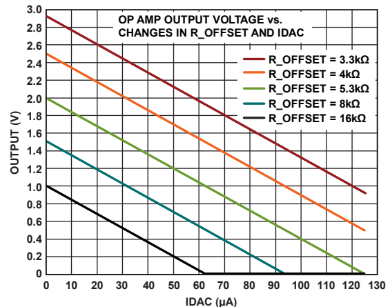
Figure 92. AUXDAC Op Amp Output vs. Current, AVDD = 3.3 \text{ V} No Load, AUXDAC 0x1FF to 0x000
