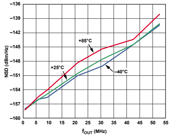
Figure 65. NSD at 8 mA, 3.3 V
