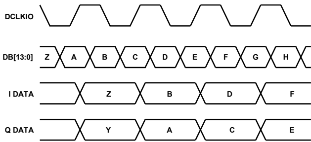
Figure 76. Timing Diagram with IFIRST = 0, IRISING = 0
