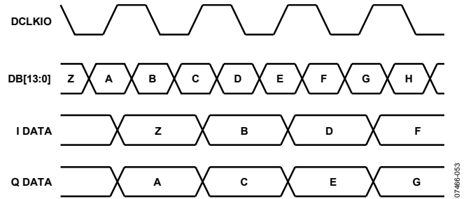
Figure 78. Timing Diagram with IFIRST = 1, IRISING = 0
