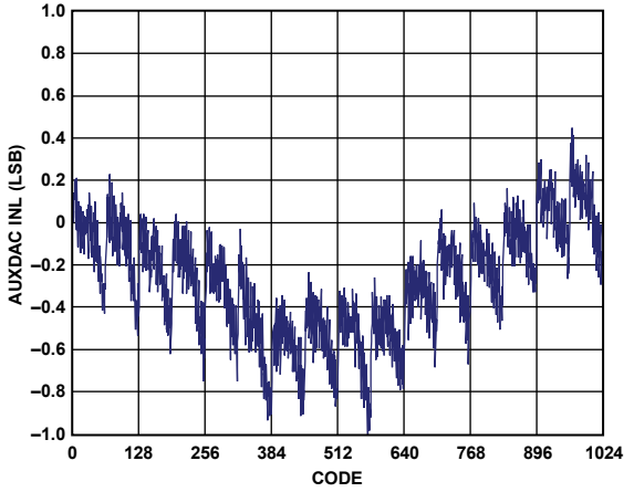
Figure 37. AUXDAC INL
