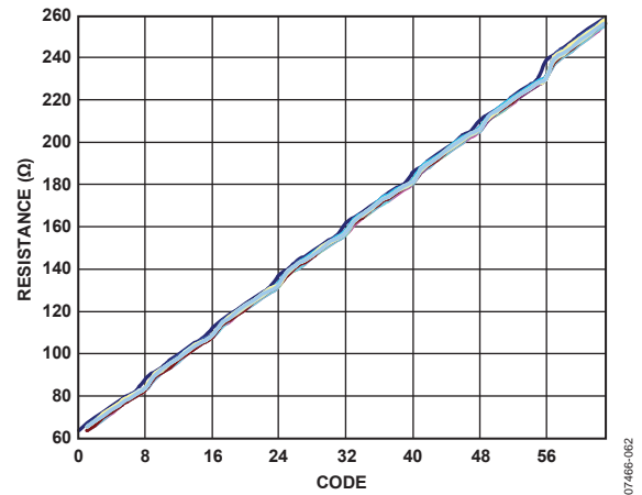
Figure 87. Typical CML Resistor Value vs. Register Code
