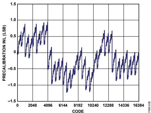
Figure 8. AD9117 Precalibration INL at 3.3 V, 20 mA
