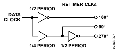
Figure 82. RETIMER-CLK Phases
