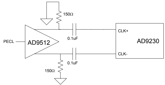
Figure X. Differential PECL Sample Clock for AD9230/AD9211
