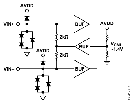
Figure 34. Analog Inputs ( V_{CML} = \sim 1.4 V )
