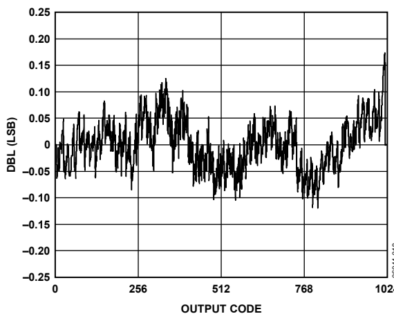
Figure 11. AD9211-200 INL; 200 MSPS
