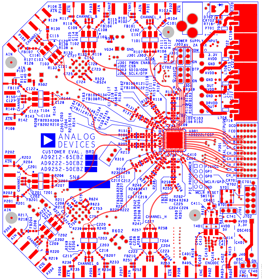
Figure 83. Evaluation Board Layout, Primary Side
