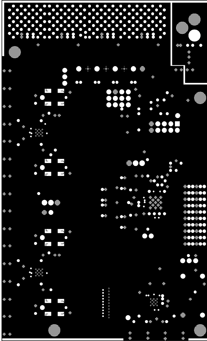
Figure 78. Evaluation Board Layout, Ground Plane
