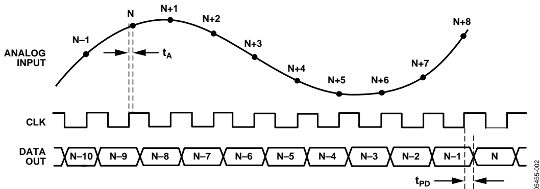
Figure 2. Timing Diagram
