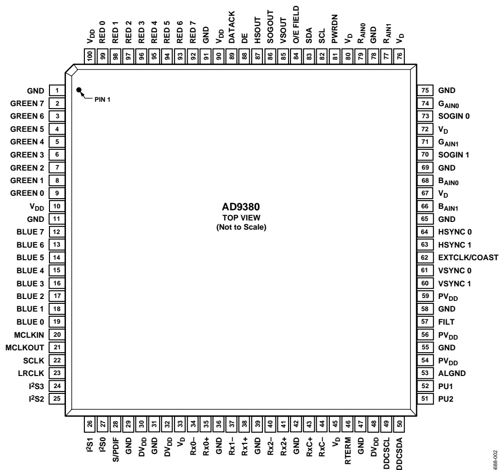
Figure 2. Pin Configuration
