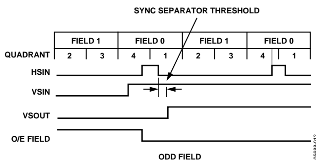
Figure 12. VSYNC Filter—Odd
