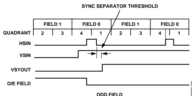
Figure 5. VSYNC Filter—Odd/Even
