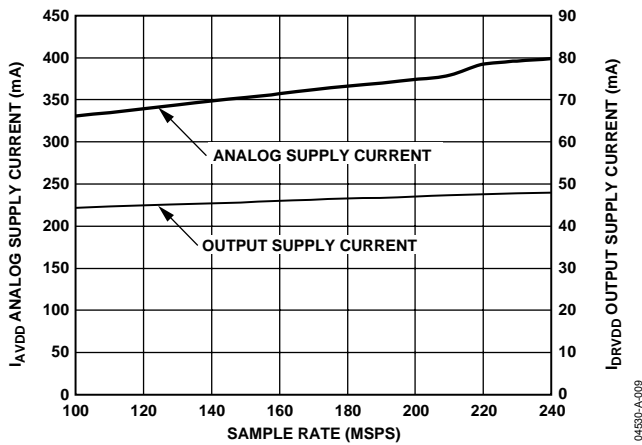
Figure 22. I AVDD and I IDRVD vs. Clock Rate, 200 MSPS Grade, CLOAD = 5 pF (AIN = 10.3 MHz @ -0.5 dBFS)
