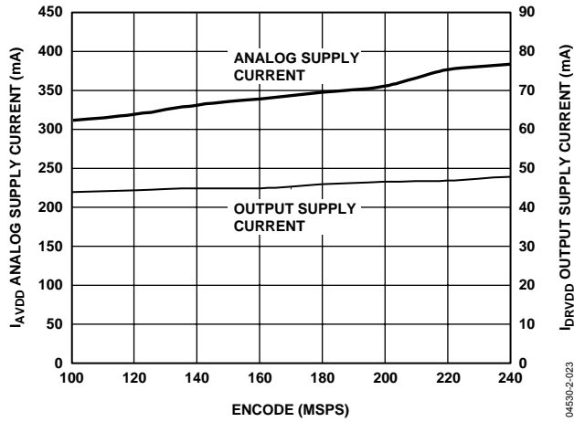
Figure 21. I AVDD and I IDRVD vs. Clock Rate, 170 MSPS Grade, CLOAD = 5 pF (AIN = 10.3 MHz @ -0.5 dBFS)
