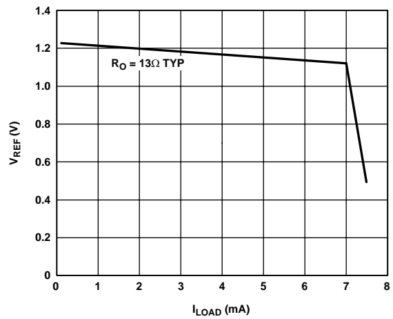
Figure 25. V REFOUT vs. I LOAD (Both Speed Grades)
