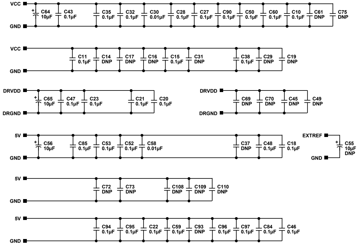
Figure 52. Evaluation Board Schematic, Bypass Capacitors
