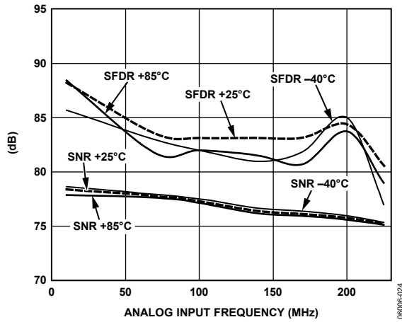
Figure 24. 105 MSPS, SNR/SFDR vs. Analog Input Frequency, 3.4 V p-p
