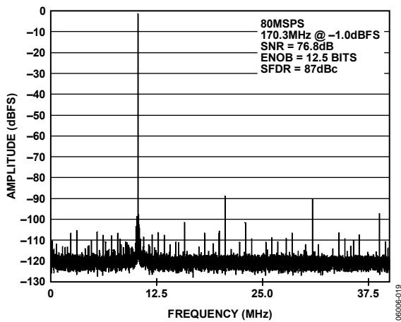
Figure 19. 80 MSPS, 64k Point, Single-Tone FFT, 170.3 MHz
