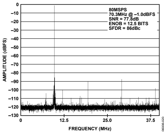
Figure 20. 80 MSPS, 64k Point, Single-Tone FFT, 70.3 MHz
