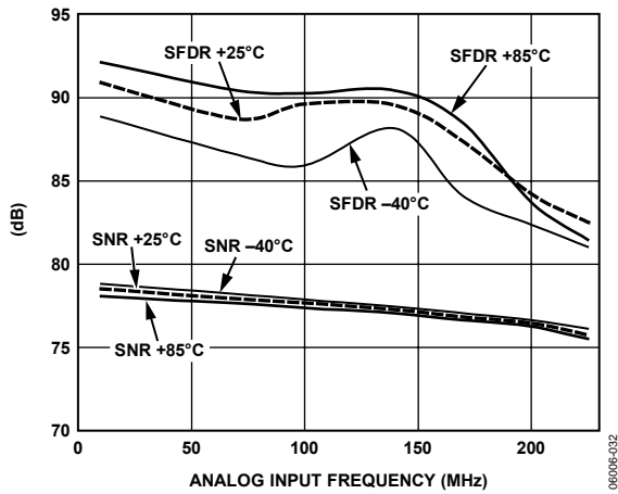
Figure 31. 80 MSPS, SNR/SFDR vs. Analog Input Frequency, 3.4 Vp-p
