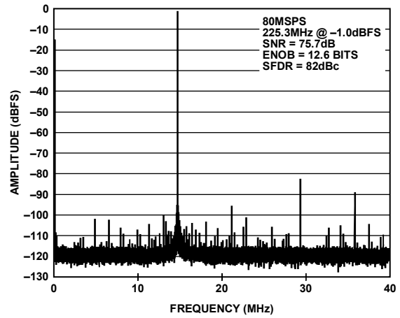
Figure 21. 80 MSPS, 64k Point Single-Tone FFT, 225.3 MHz
