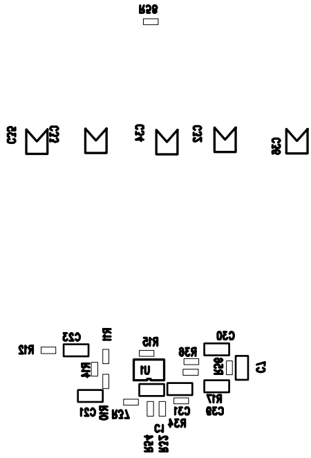
Figure 46. PCB Bottom-Side Silkscreen
