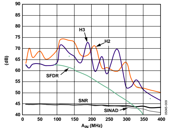
Figure 9. Analog Input Frequency Sweep, A_{IN} = -1 dBFS, FS = 0.75 V, f_s = 250 MSPS, External VREF Mode
