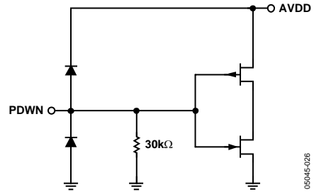
Figure 26. Power-Down Input
