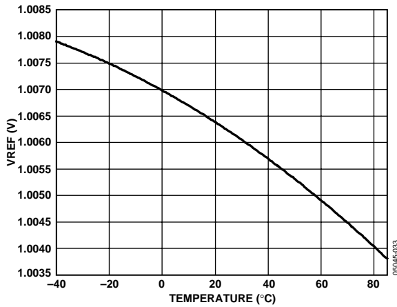
Figure 32. Typical Reference Variation with Temperature
