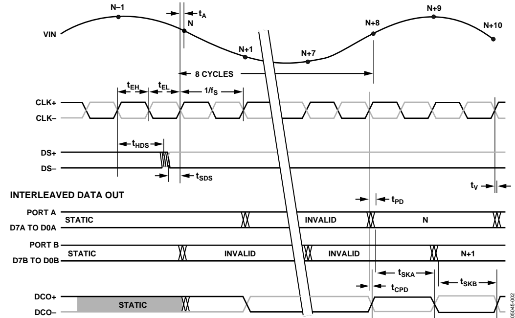
Figure 2. Timing Diagram
