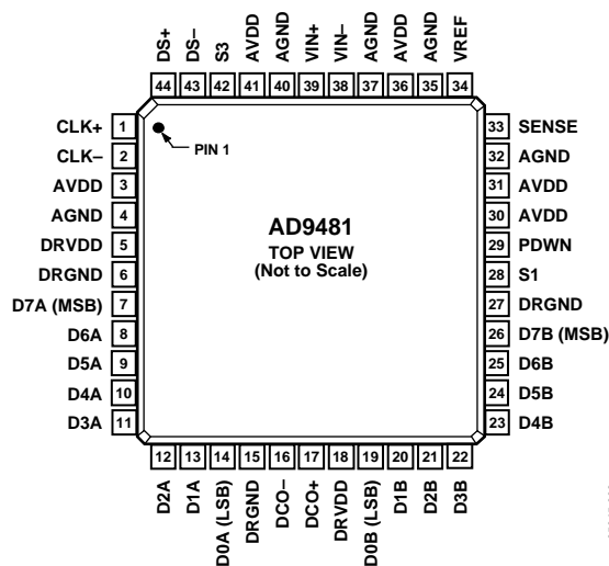
Figure 3. Pin Configuration
