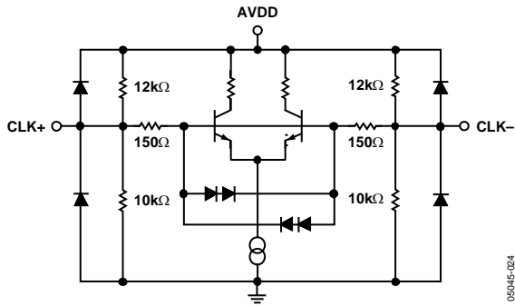
Figure 24. Clock Inputs
