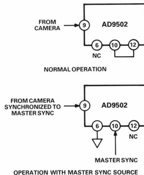
Figure 4. Monochrome Operation
