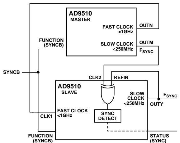
Figure 43. Multichip Synchronization
