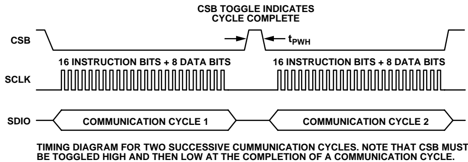
Figure 52. Use of CSB to Define Communications Cycle
