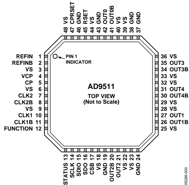
Figure 6. 48-Lead LFCSP Pin Configuration
