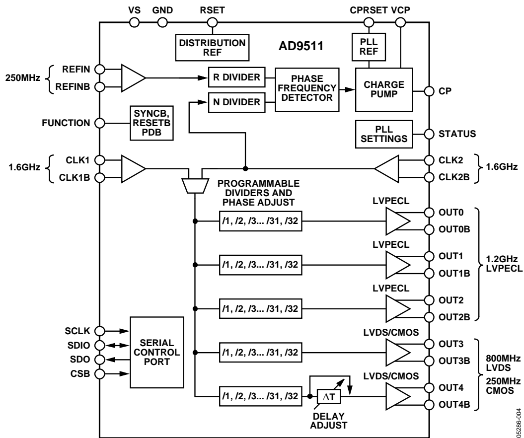
Figure 33. Functional Block Diagram Showing Maximum Frequencies
