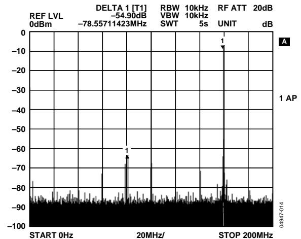
Figure 15. AD9540 DAC Performance: 400 MSPS Clock, 160 MHz F_{OUT} , 200 MHz Span
