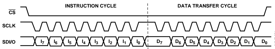
Figure 38. Serial Port Write Timing—Clock Stall High
