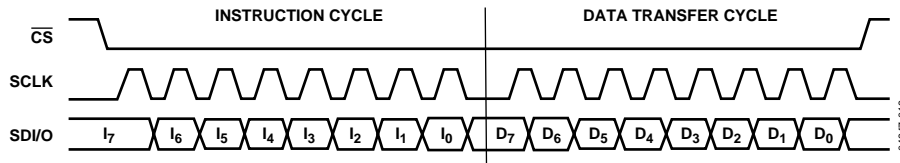
Figure 36. Serial Port Write Timing—Clock Stall Low
