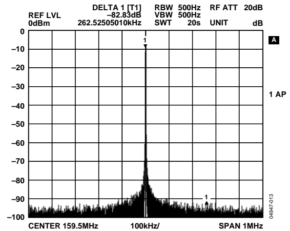
Figure 14. AD9540 DAC Performance: 400 MSPS Clock, 160 MHz F_{OUT} , 1 MHz Span
