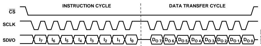
Figure 39. 2-Wire Serial Port Read Timing—Clock Stall High
