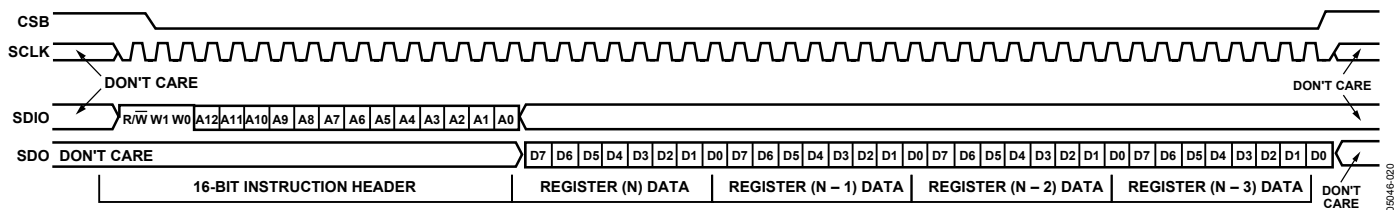
Figure 40: Serial Control Port Read—MSB First, 16-Bit Instruction, 4 Bytes Data
