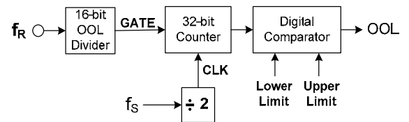
Figure 18: Reference Monitor
