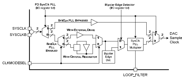
Figure 28: System Clock Generator Block Diagram
