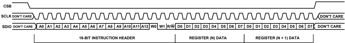
Figure 43: Serial Control Port Write—LSB First, 16-Bit Instruction, 2 Bytes Data
