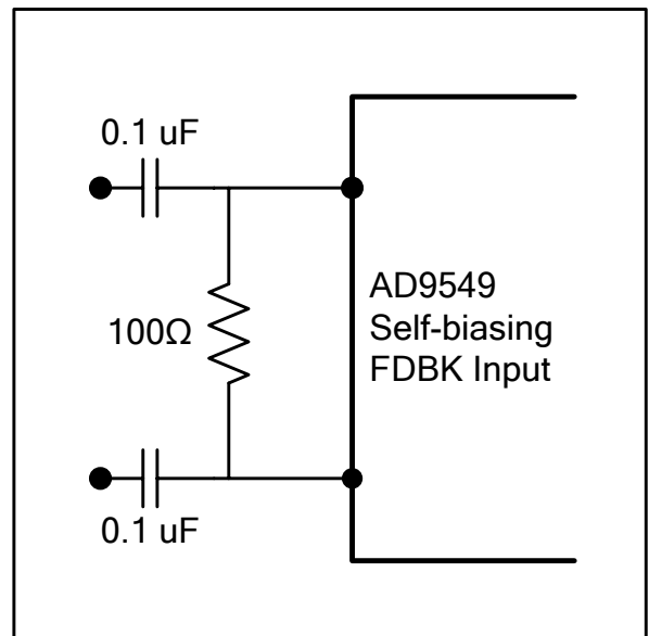
Figure 7: FDBK Input.
