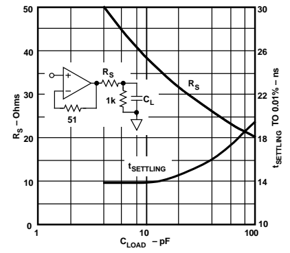
Figure 15. Settling Time vs. Capacitive Load
