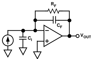
Figure 1. Transimpedance Configuration
