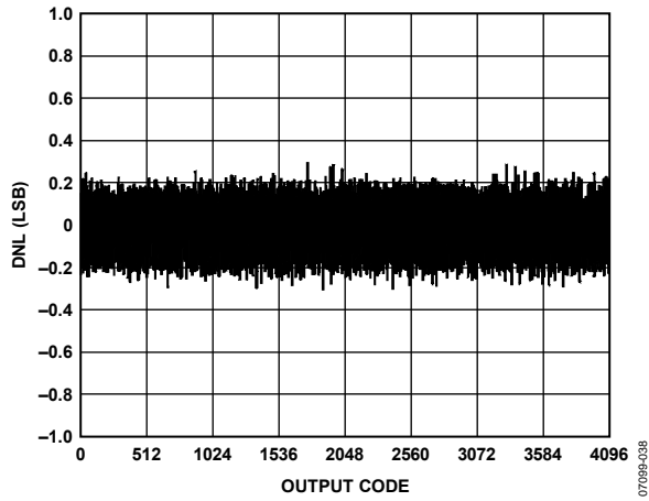
Figure 29. AD9626-210 DNL; 210 MSPS
