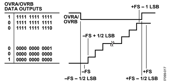
Figure 51. OVRA/OVRB Relation to Input Voltage and Output Data
