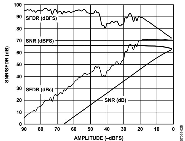
Figure 16. AD9626-170 SNR/SFDR vs. Input Amplitude; 140.3 MHz
