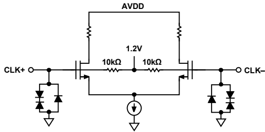
Figure 5. Clock Inputs
