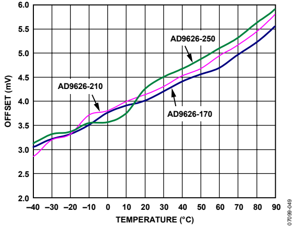
Figure 41. Offset vs. Temperature
