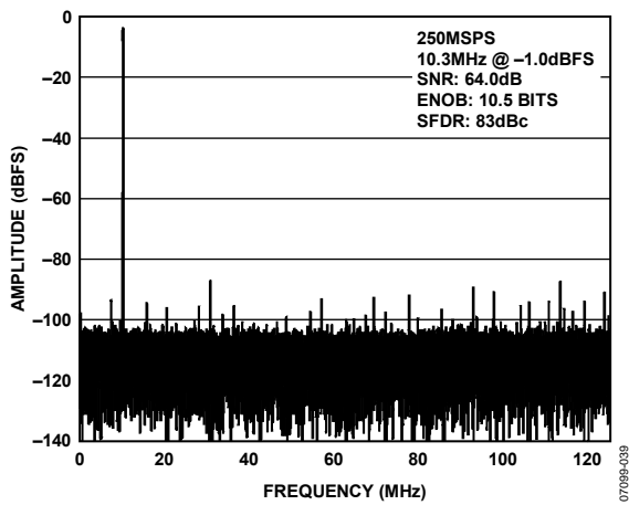
Figure 30. AD9626-250 64k Point Single-Tone FFT; 250 MSPS, 10.3 MHz
