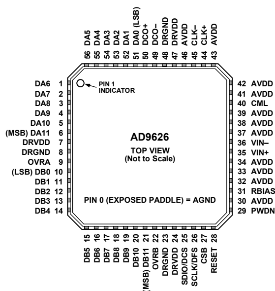
Figure 4. Pin Configuration
