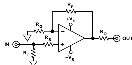
Noninverting Configuration
