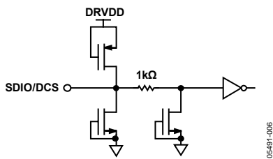
Figure 5x. Equivalent SDIO/DCS Input Circuit
