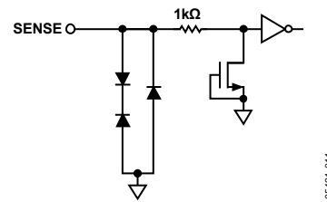
Figure 7. Equivalent SENSE Circuit
