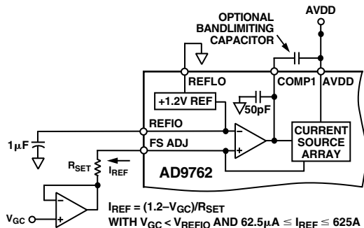
Figure 44. Dual-Supply Gain Control Circuit
