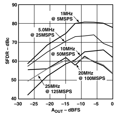
Figure 28. Single-Tone SFDR vs. A_{OUT} @ f_{OUT} = f_{CLOCK}/5
