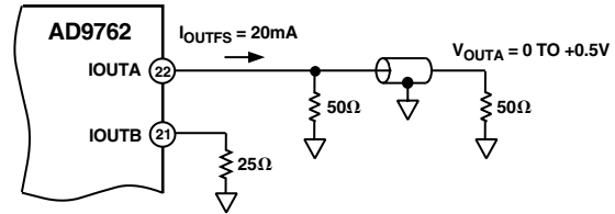
Figure 53. 0\text{ V} to +0.5\text{ V} Unbuffered Voltage Output
