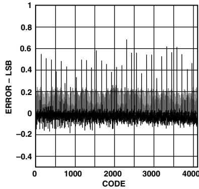
Figure 34. Typical DNL
