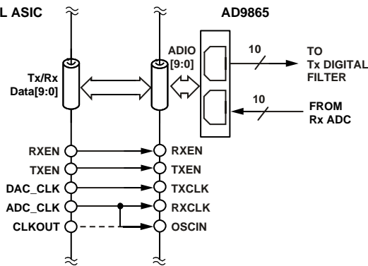
Figure 51. Example of a Half-Duplex Digital Interface with AD9865 Serving as the Slave
