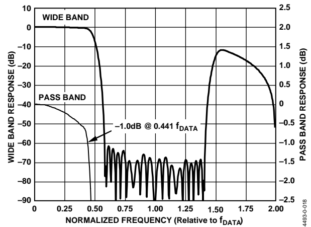
Figure 60. Frequency Response of 2\times Interpolation Filter (Normalized to f_{DATA} )
