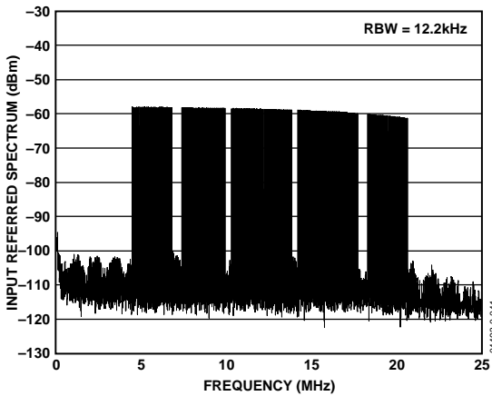
Figure 4. Spectral Plot with 4 k FFT of 84-Carrier DMT Signal with PAR = 10.2 dB, P_{IN} = -33.7 dBm, and RxPGA = 36 dB
