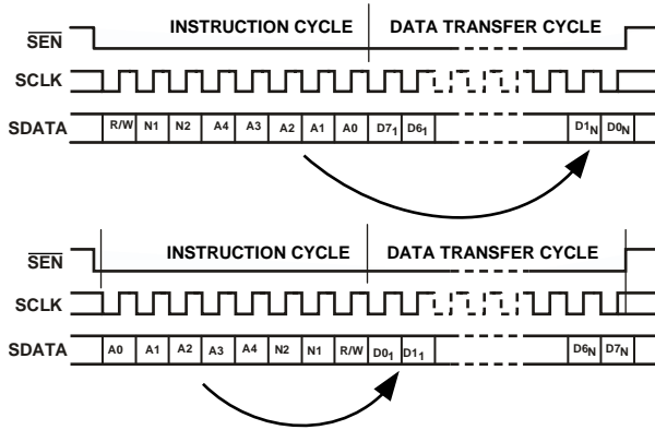
Figure 45. SPI Timing, MSB First (Upper), and LSB First (Lower)
