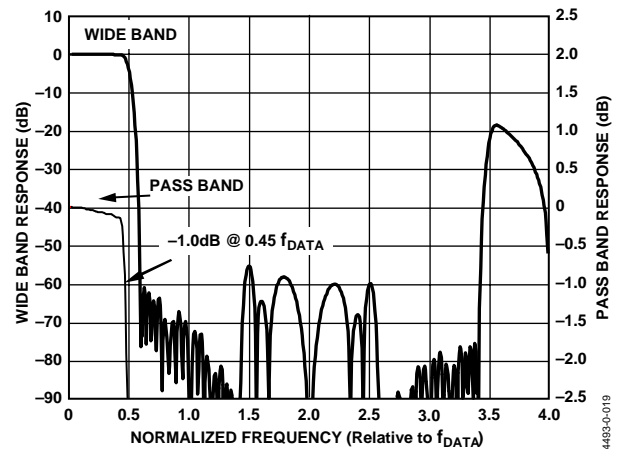
Figure 61. Frequency Response of 4\times Interpolation Filter (Normalized to f_{DATA} )
