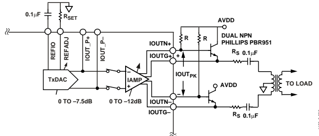
Figure 65. Voltage-Mode Operation
