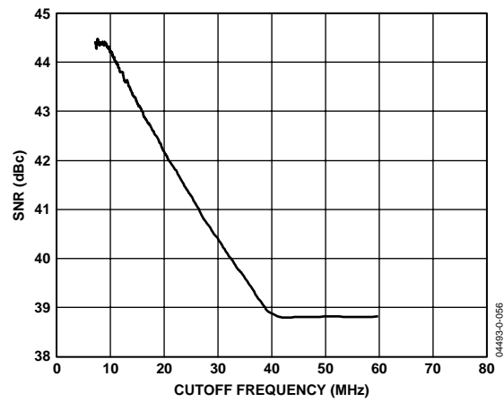
Figure 19. SNR vs. Filter Cutoff Frequency (50 MSPS; f_{IN} = 5 MHz; A_{IN} = -1 dB; RxPGA = 48 dB)
