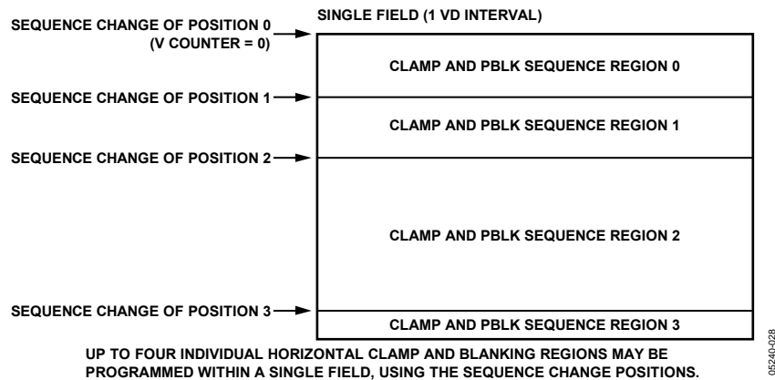
Figure 25. CLPOB and PBLK Sequence Flexibility
