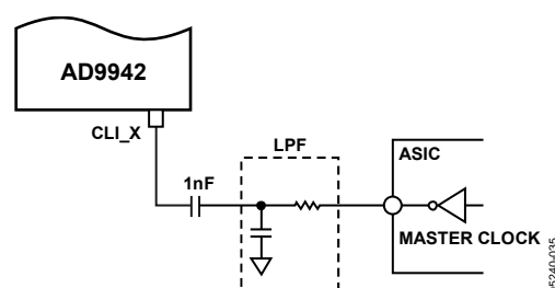
Figure 32. CLI Connection, AC-Coupled
