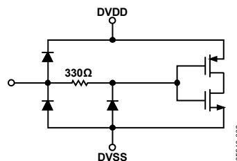
Figure 6. Digital Inputs
