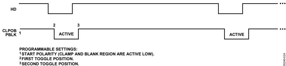
Figure 21. CLPOB and PBLK Pulse Placement
