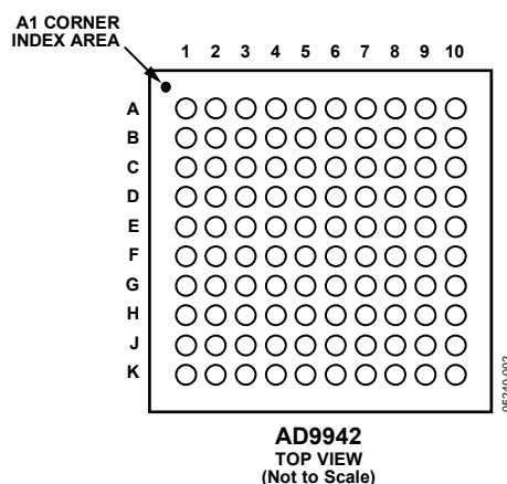
Figure 2. Pin Configuration
