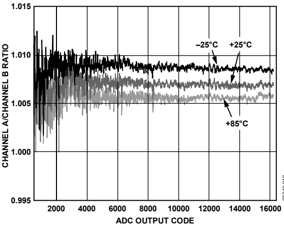
Figure 10. Noncalibrated Channel A/Channel B Ratio
