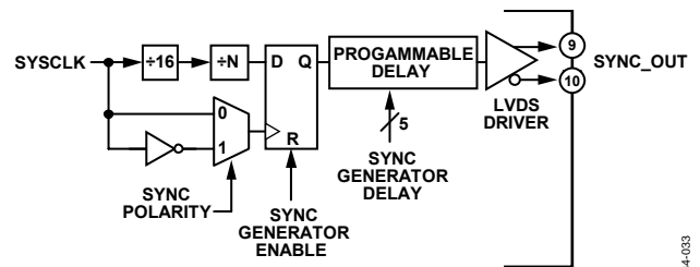
Figure 55. Sync Generator
