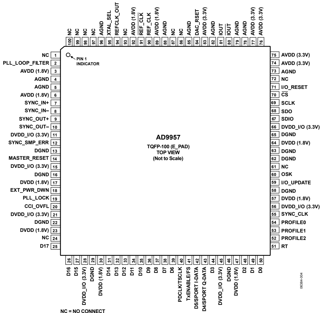
Figure 4. Pin Configuration
