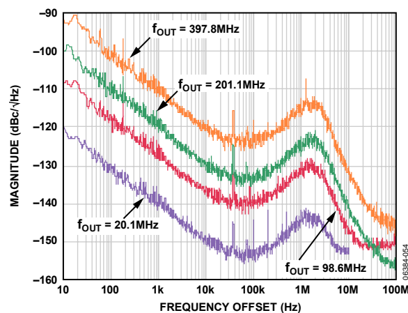
Figure 21. Residual Phase Noise Using the REFCLK Multiplier, REFCLK = 50 MHz with 20x Multiplication, System Clock = 1 GHz
