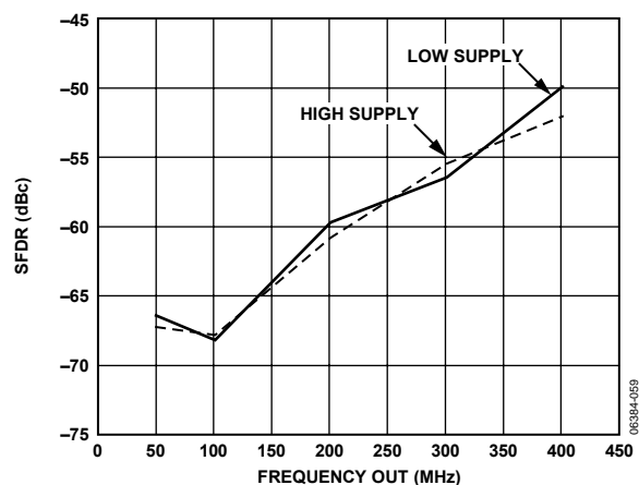
Figure 18. SFDR vs. Output Frequency vs. Supply ( \pm 5\% ) in Single Tone Mode
