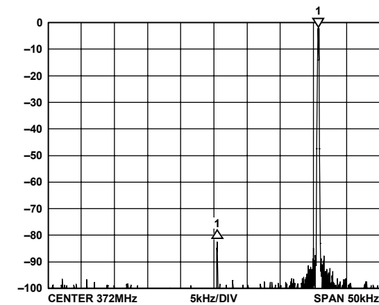
Figure 10. Narrow-Band View of Figure 7 (with Carrier and Lower Sideband Suppression)
