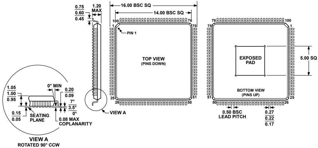
Figure 63. 100-Lead Thin Quad Flat Package, Exposed Pad [TQFP_EP] (SV-100-4) Dimensions shown in millimeters
