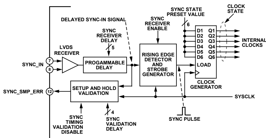
Figure 56. Sync Receiver
