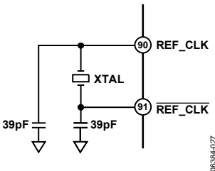
Figure 48. Crystal Connection Diagram
