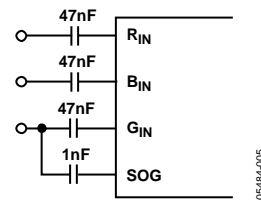
Figure 5. Typical Clamp Configuration
