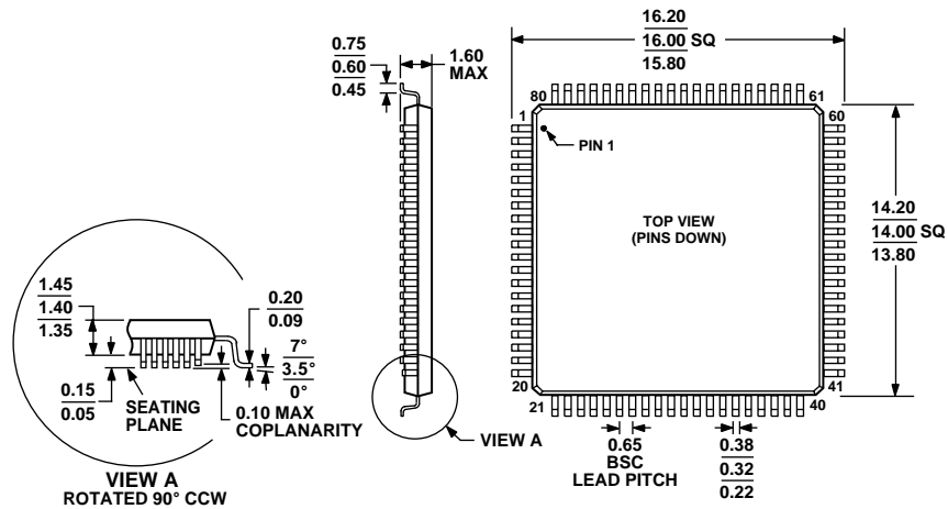
Figure 16. 80-Lead Low Profile Quad Flat Package [LQFP] (ST-80-2)
