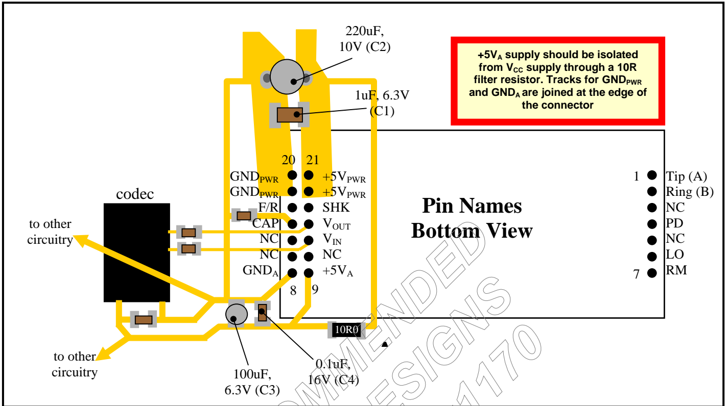
Figure 6: Layout Considerations.
