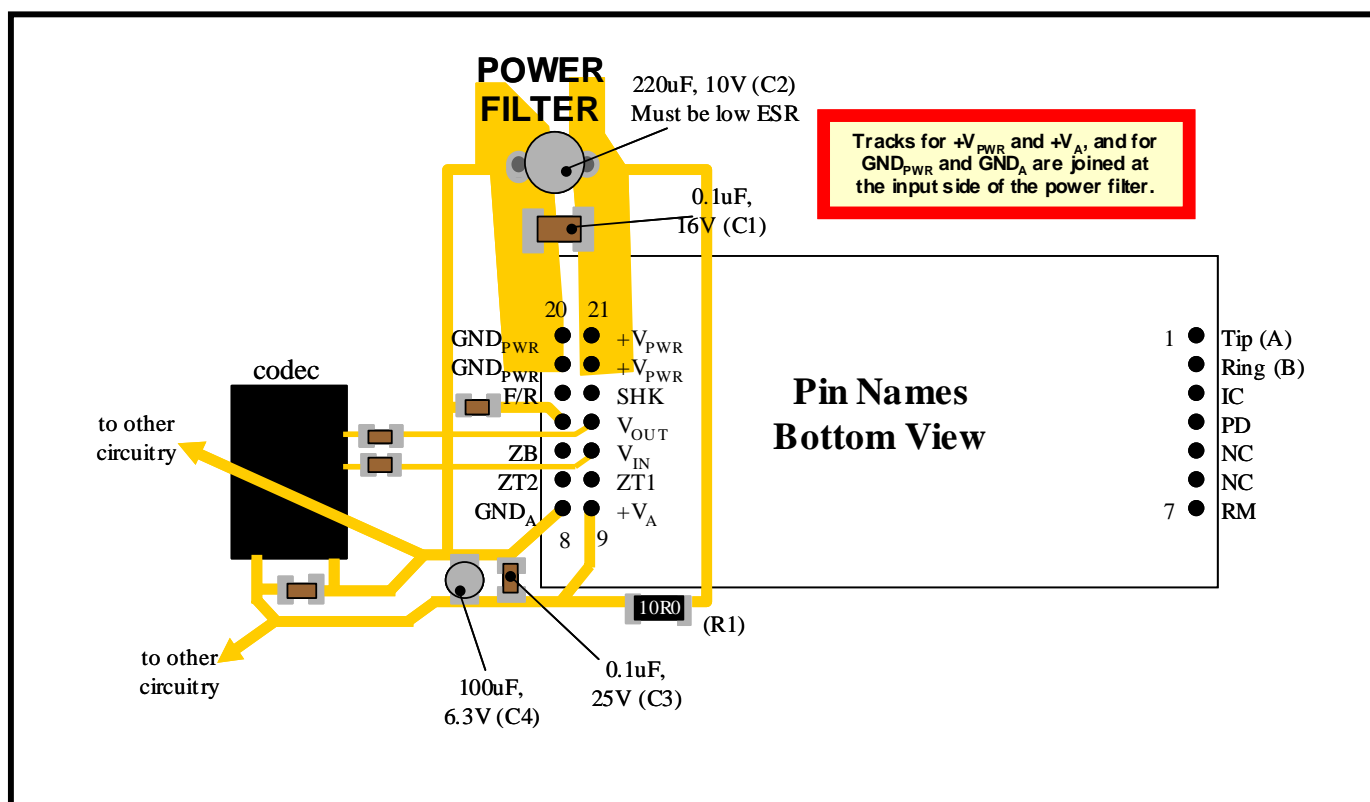
Figure 7: Typical Layout
