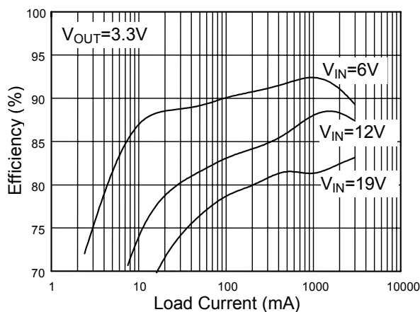
Fig. 1 Efficiency vs Load Current ( V_{OUT}=3.3V )
