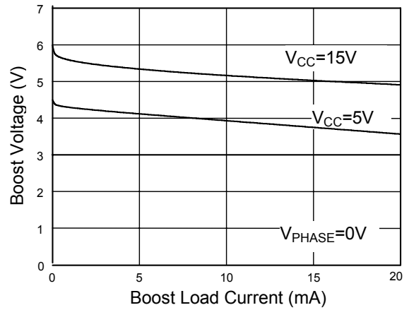
Fig. 6 Boost Load Regulation
