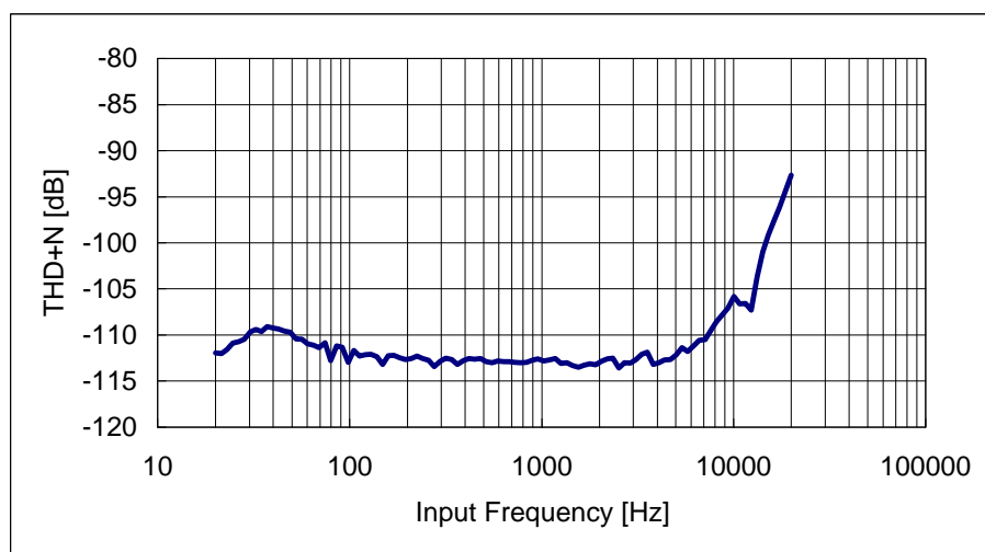
Figure 2: Input Frequency vs. THD+N (FSI=44.1kHz, FSO=48kHz)
