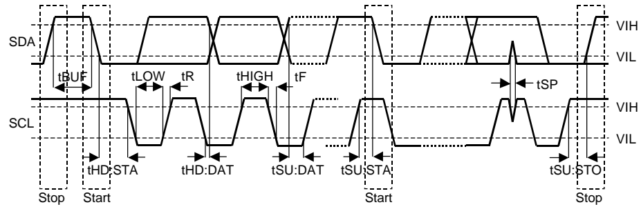
I²C Bus mode Timing
