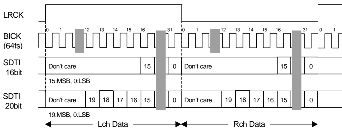
Figure 7. LSB justified Timing
