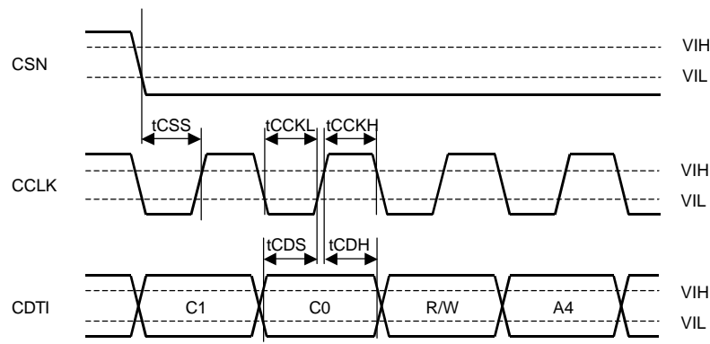
WRITE Command Input Timing (3-wire Serial mode)
