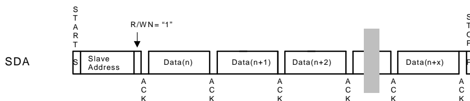
Figure 15. CURRENT ADDRESS READ
