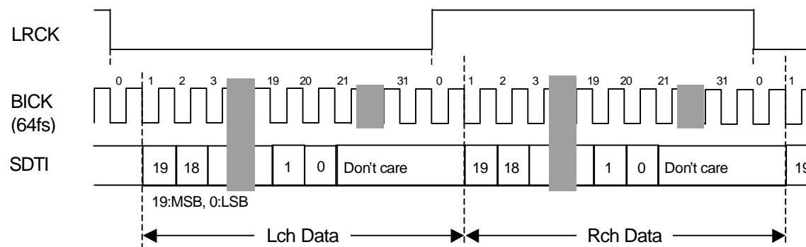
Figure 9. I 2 S Timing
