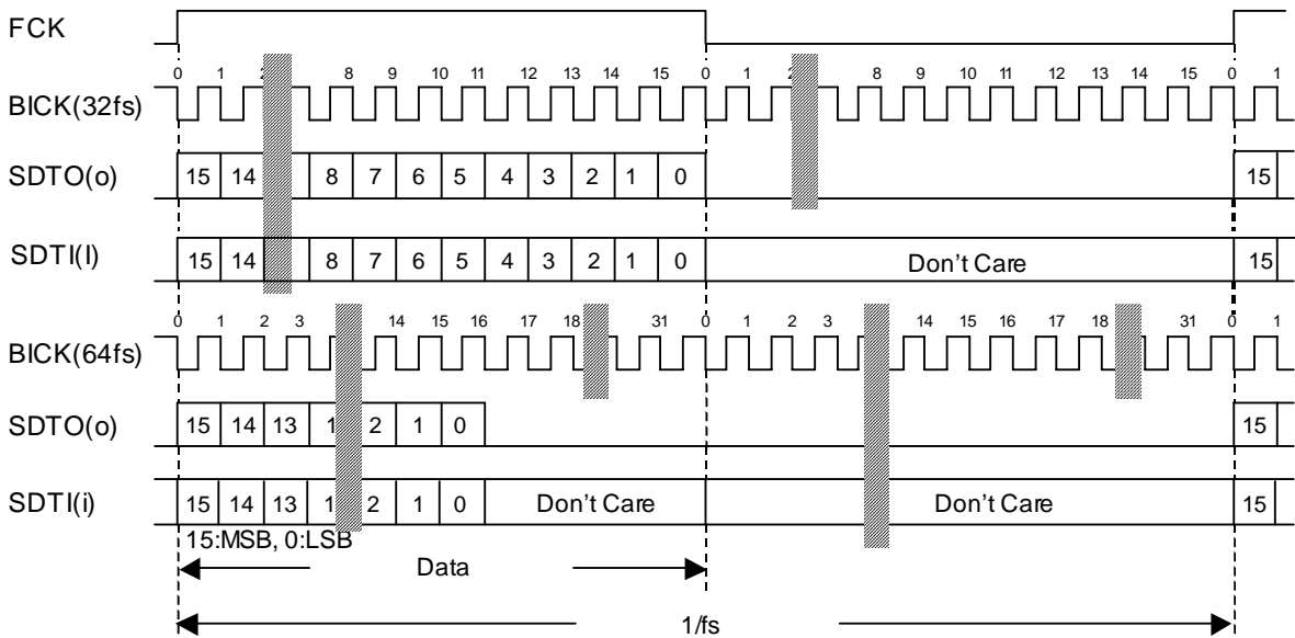
Figure 28. Mode 2 Timing
