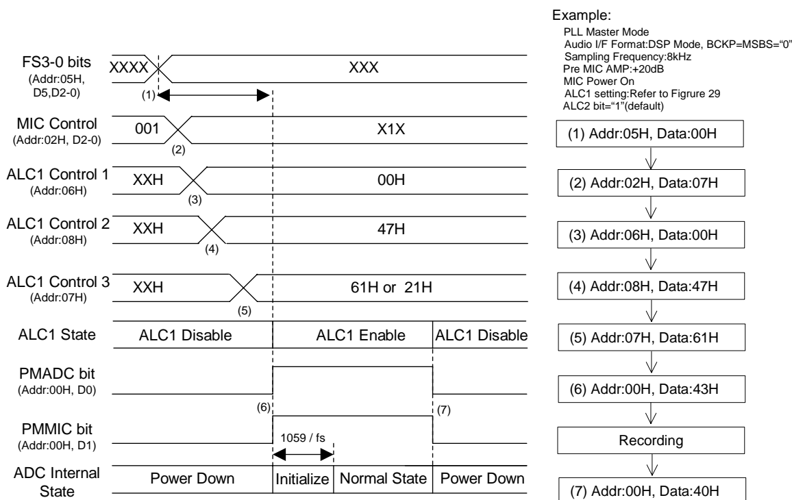
Figure 50. MIC Input Recording Sequence
