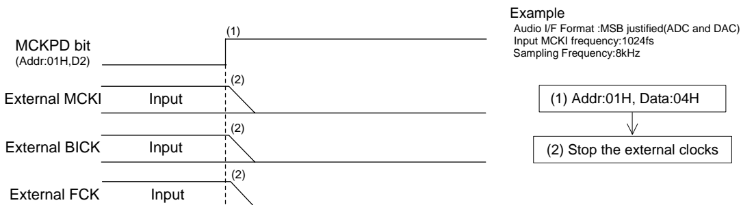
Figure 59. Clock Stopping Sequence (4)
