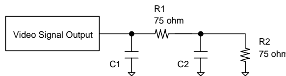
Figure 2. Load Capacitance C1 and C2
