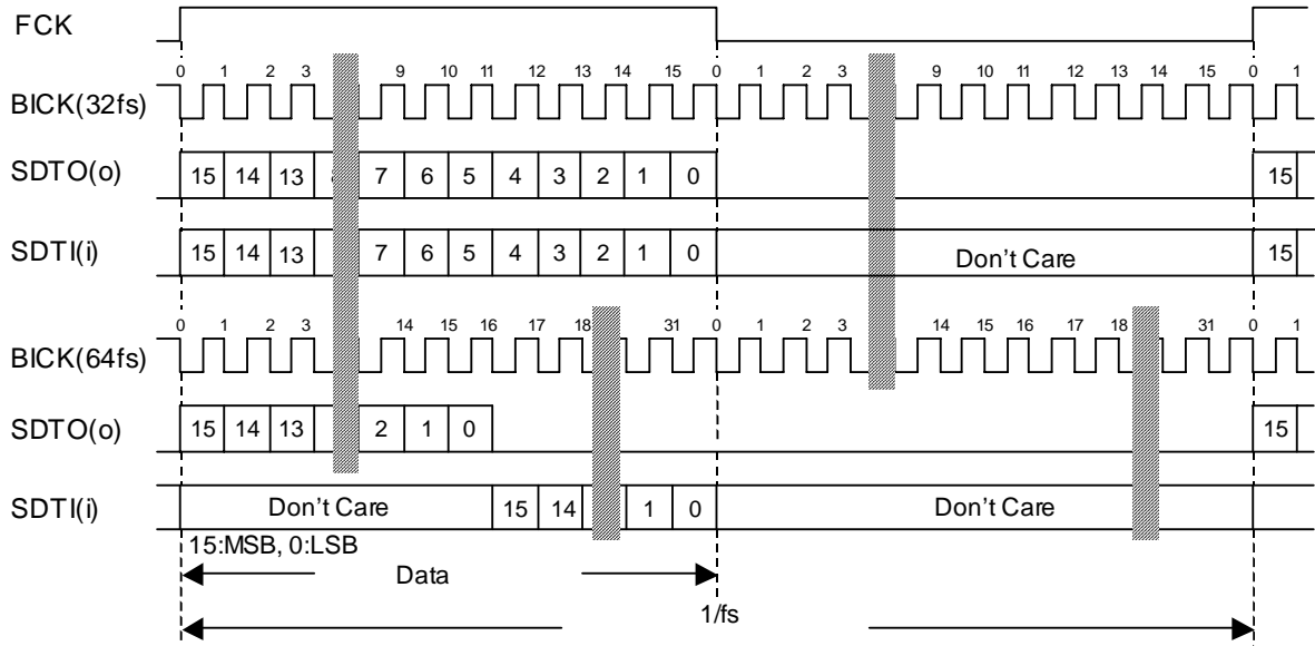
Figure 27. Mode 1 Timing
