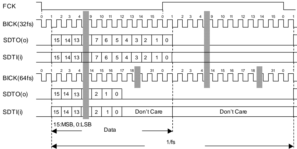
Figure 29. Mode 3 Timing
