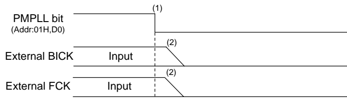
Figure 57. Clock Stopping Sequence (2)
