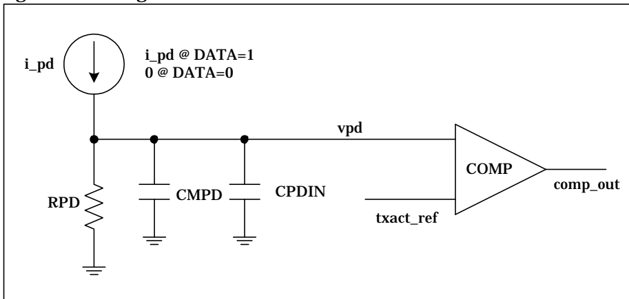
Fig 3-2 Reference figures for TXACT detection time
