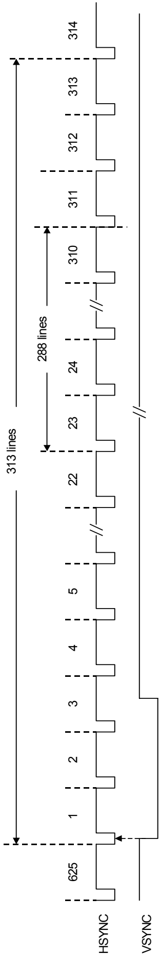
( 2 ) PAL ( Frame ) 625 Line 576 active lines The First Field ( ODD )
