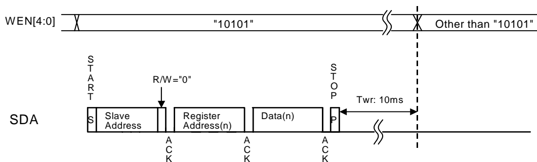
Fig. 12 Byte-write
