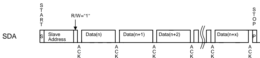
Fig. 08 CURRENT ADDRESS READ
