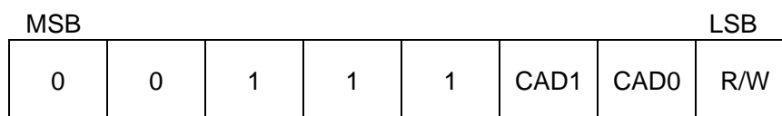
Fig. 04 Slave Address
