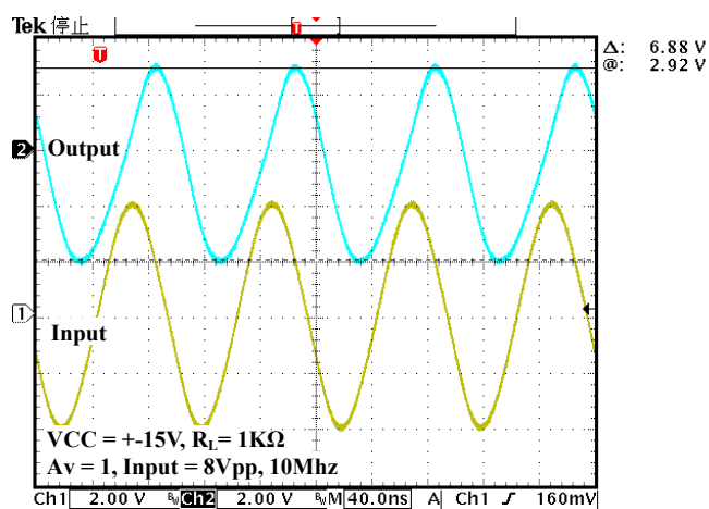
Large signal Output Swing at 10Mhz, A_v=1
