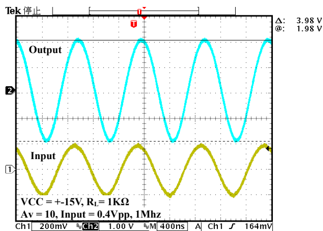
Output Swing at 1Mhz, A_v=10
