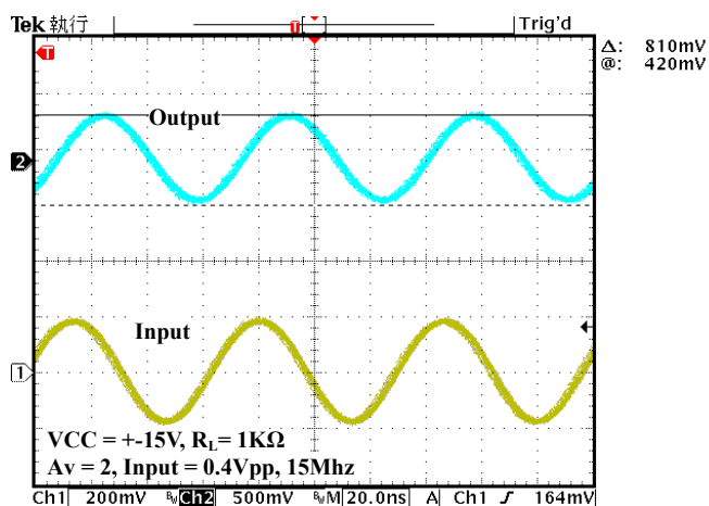
Output Swing at 15Mhz, A_v=2
