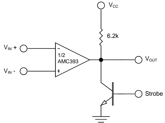
Output Strobing
