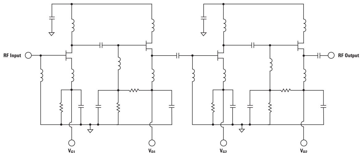
Figure 19. AMMC-5023 Schematic.
