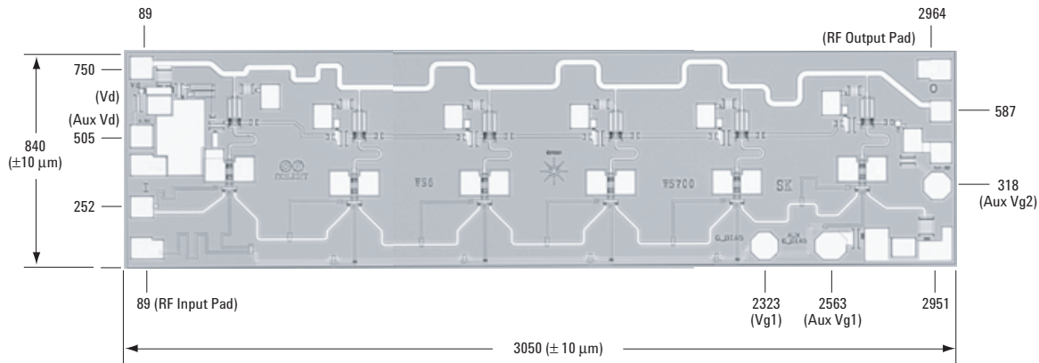
Figure 16. AMMC-5026 Bonding Pad Locations. (dimensions in micrometers)
