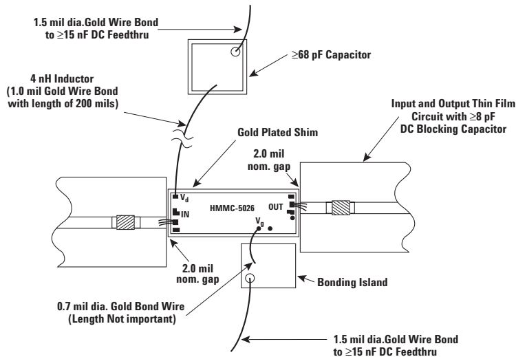
Figure 17. AMMC-5026 Assembly Diagram.
