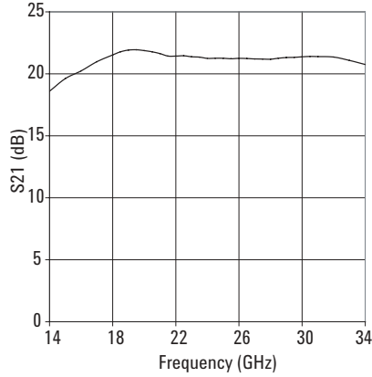
Figure 1. Typical Gain
