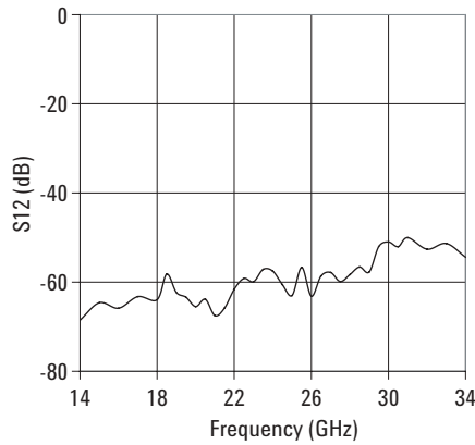
Figure 2. Typical Isolation
