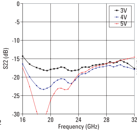
Figure 14: Output Return Loss Over Vdd
