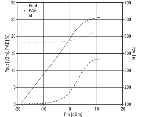
Figure 6. Typical Output Power, PAE, and Total Drain Current versus Input Power at 30GHz
