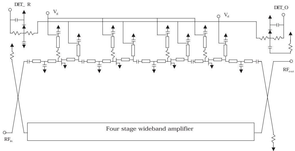
Figure 11. AMMC-6345 Schematic
