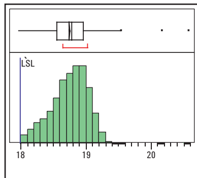
Gain at 30 GHz
