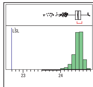
P-1dB at 38 GHz
