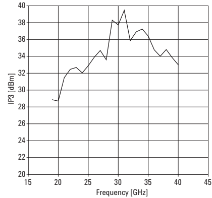
Figure 5. Typical Output 3 rd Order Intercept Pt.
